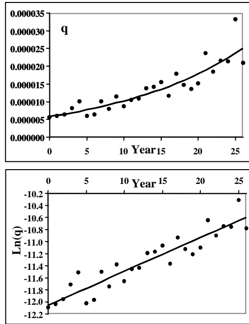
Figure A10.1. The top panel is the final distribution of expected catchability coefficients with the fitted curve of form Eq. A.24. In order to estimate the two parameters q_0 and q_{\text{inc}} instead of a simple geometric average of the expected q values we have to fit the curve. By log-transforming each q_t value and plotting these against the number of times the q_{\text{inc}} is applied to the starting value a straight line is obtained as in the lower panel. The straight line is defined by Eq. A.25, so the two parameters may be determined by anti-logging the two parameters from the linear regression. Data is a bootstrap sample from the northern Australian tiger prawn fishery (see Example Box 10.6).
