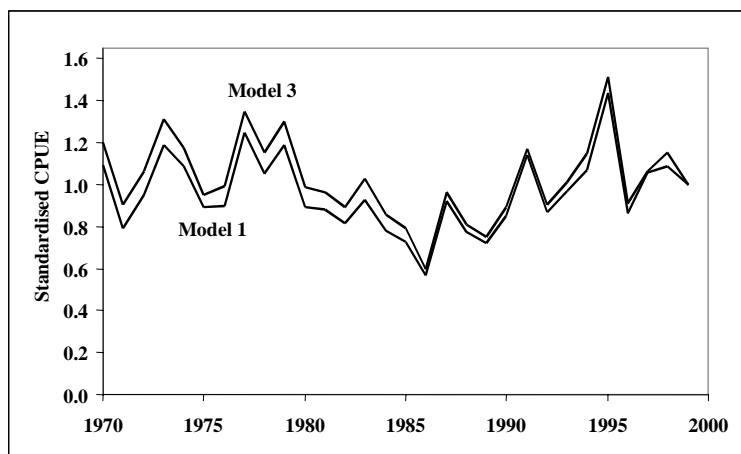
Fig. 5.3 Standardised CPUE for the Northern prawn fishery relative to 1999. Model 1 represents the unstandardized geometric means of the selected raw data. Model 3 is a sub-optimal model \ln(CE) = \text{Constant} + \text{Year} + \text{Month} + \text{Week} (see Table 5.2; and cf. Fig. 5.2).
